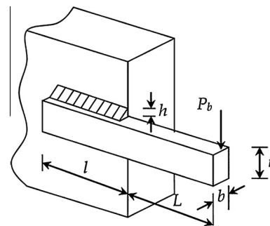
Fig. 10. Schematic of welded beam design problem.
